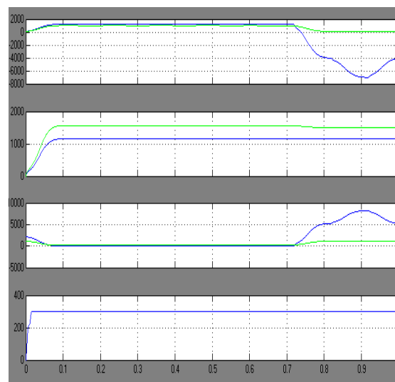
Fig.8. Simulation results a) PQ-grid, b) PQ-load, c) PQ - inv, d) dc link voltage under no voltage variations from RES
