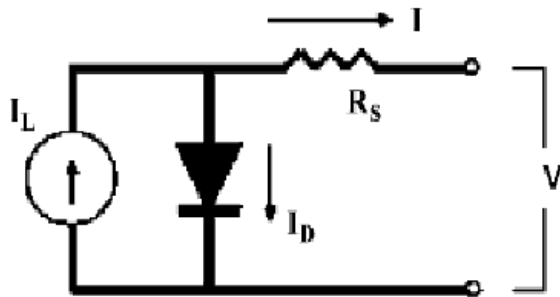
Fig 4. Solar-Cell Equivalent Circuit.
