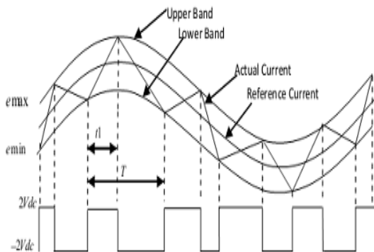
Fig 3. Waveform of Hysteresis current controller
