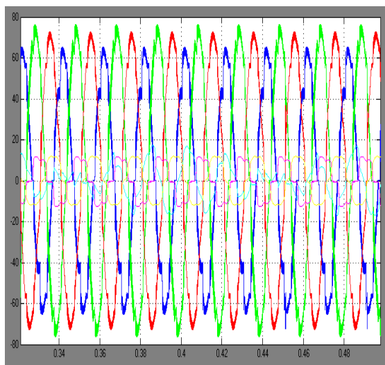
Fig.9 Load side Output wave form with hybrid filter
