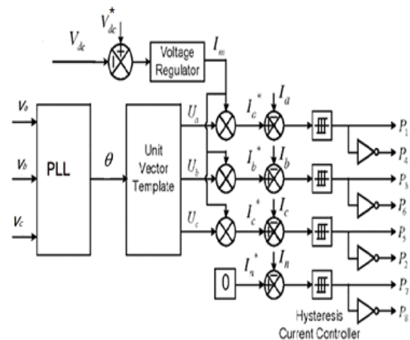
Fig 2. Control Scheme
