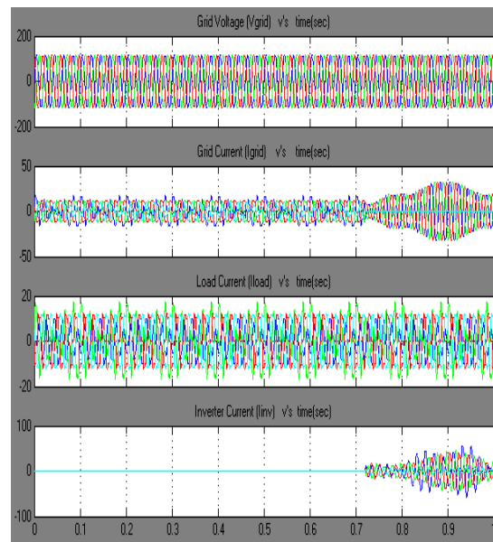
Fig.7. simulation results a) grid voltages, b) grid currents, c) load currents, d) inverter currents using PI controller
