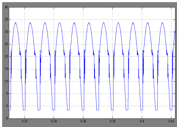
Fig. 6 Simulation results power factor for Unbalanced Nonlinear Load
