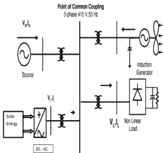
Fig.1 Single line diagram for Hybrid system
